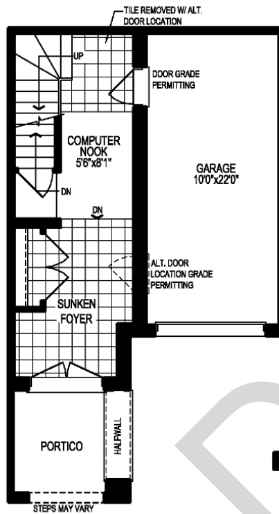
GROUND FLOOR PLAN, EL. 'A'
