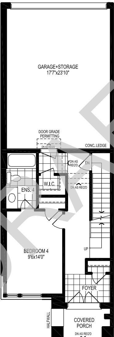
OPT. GROUND FLOOR PLAN, EL. 'C' W/ BEDROOM 4 + ENSUITE
